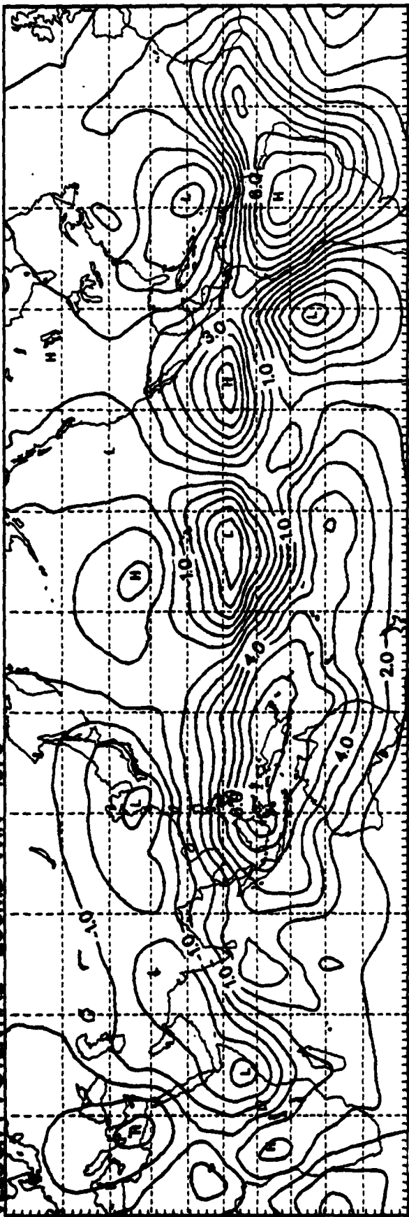
VELOCITY POTENTIAL 200MB WIN 1976
